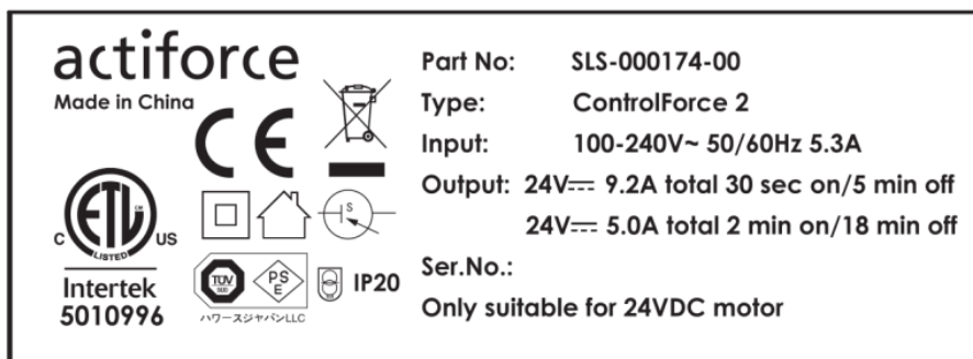
Label for adapter
