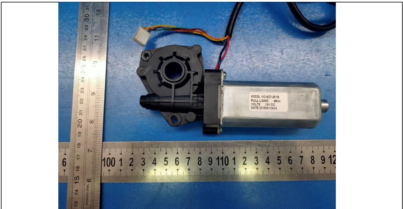
Details of: Motor(40ZYJ001B)
